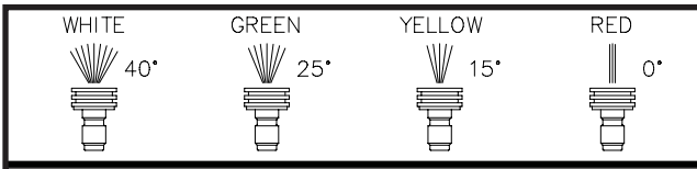
Figure 8 – Spray patterns of nozzles
